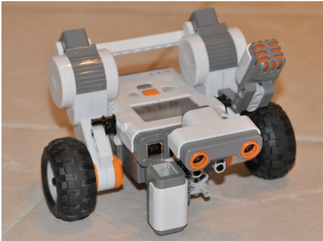
Figure 1. Configuration for Lego Mindstorms workshops: the NXT brick is mounted on a two-motor car structure (with rear swivel wheel not shown), with the following sensor modules attached: Ultrasonic Sensor, Light Sensor, Sound Sensor, Touch Sensor, Rotation sensors in two servo motors. Connector cables not shown.
