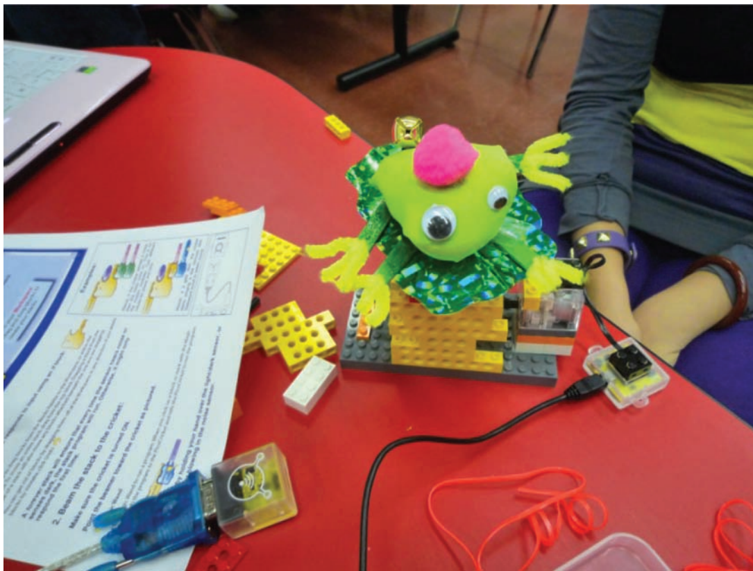
Figure A3.3. A jumping frog on a modified up-and-down motion framework.
